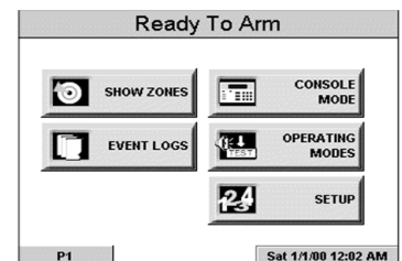
Program Screen
